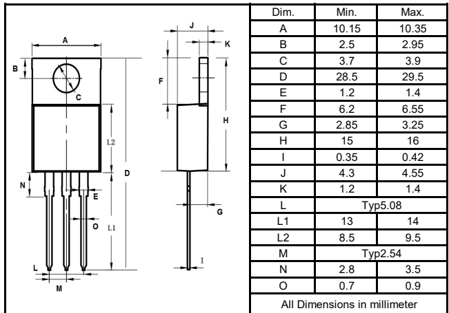
T0-220AB
